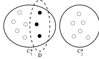
Figure 2: Illustration of Theorem 4
