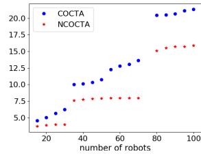
(a) SF vs number of robots on a perfect 2-ary tree ( H=15 )
