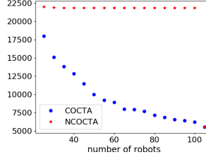
(g) Coverage time vs number of robots on a perfect 4-ary tree ( H=8 )
