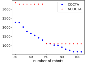
(f) Coverage time vs number of robots on a perfect 3-ary tree ( H=8 )
