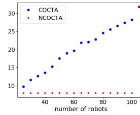
(c) SF vs number of robots on a perfect 4-ary tree ( H=8 )
