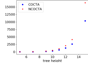
(h) Coverage time on a perfect 2-ary tree using 60 robots with different tree heights
